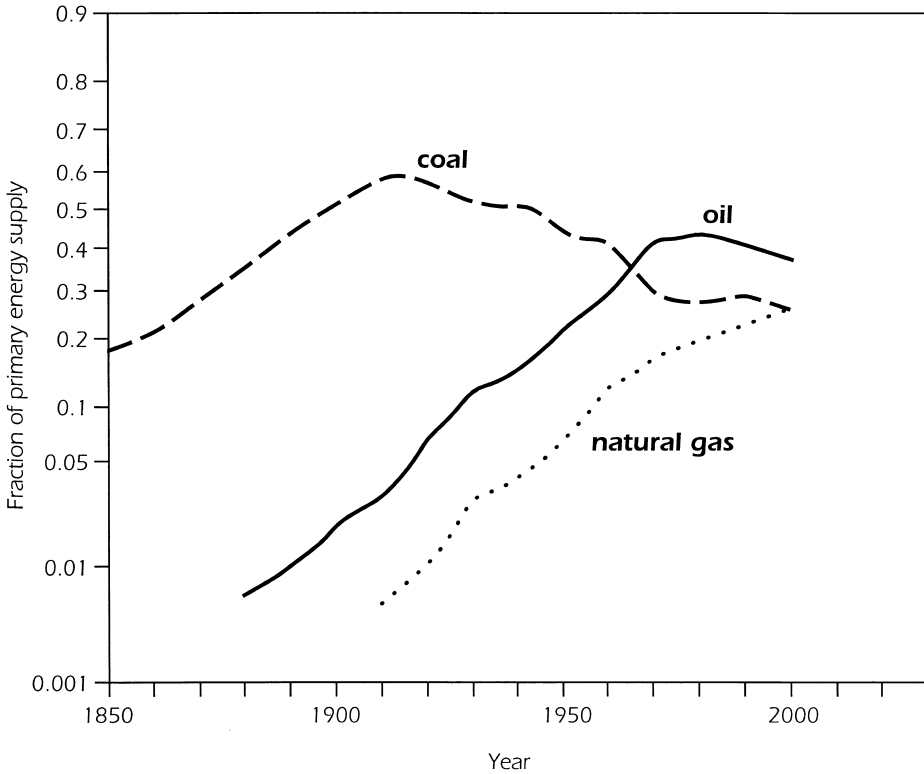
Fig. 5. Recent major departures from Marchetti's idealized system.
