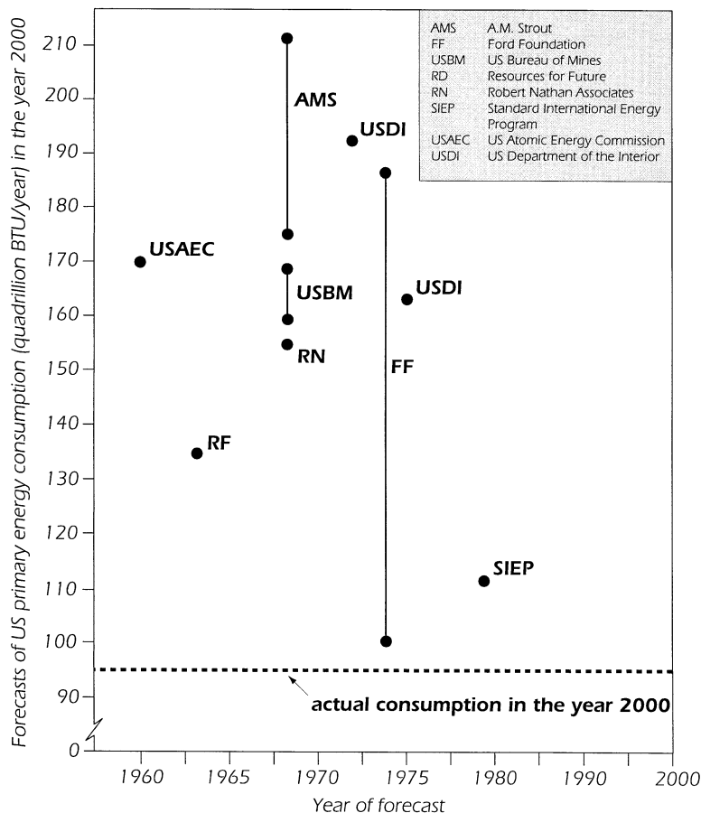
Fig. 1. Forecasts of the U.S. primary energy consumption in the year 2000.
