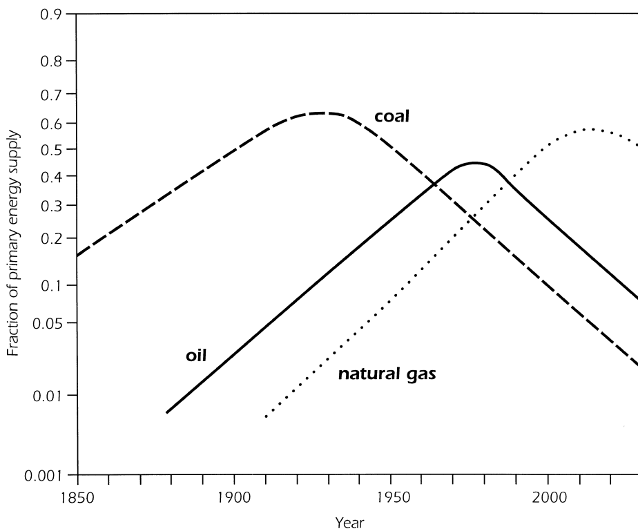
Fig. 4. Marchetti's energy substitutions working like a clock.
