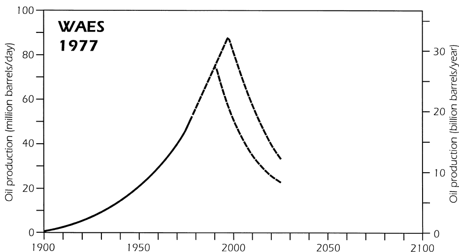
Fig. 2. Global oil exhaustion curves generated by the WAES in 1977.
