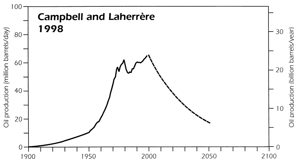
Fig. 3. Global exhaustion curve of 1750 billion barrels of liquid crude oil reserves according to Campbell and Laherrère.
